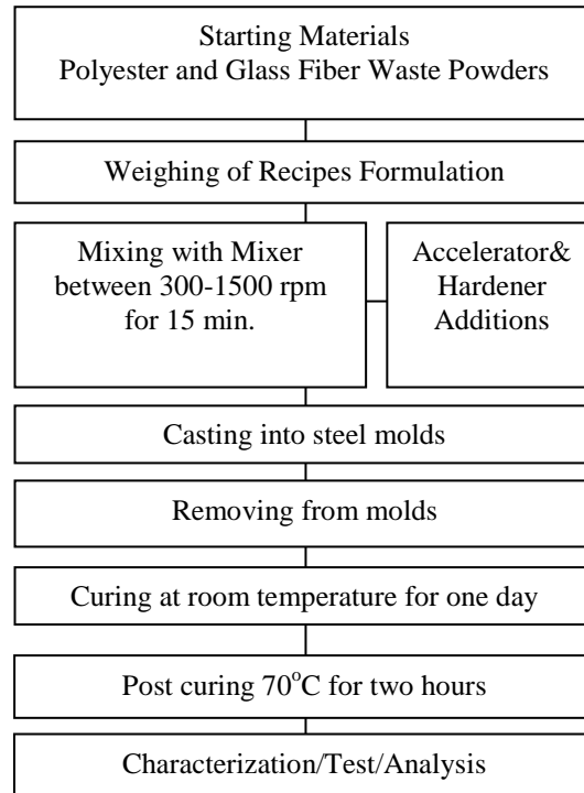
Fig-2: Polymer matrix composite preparation steps
