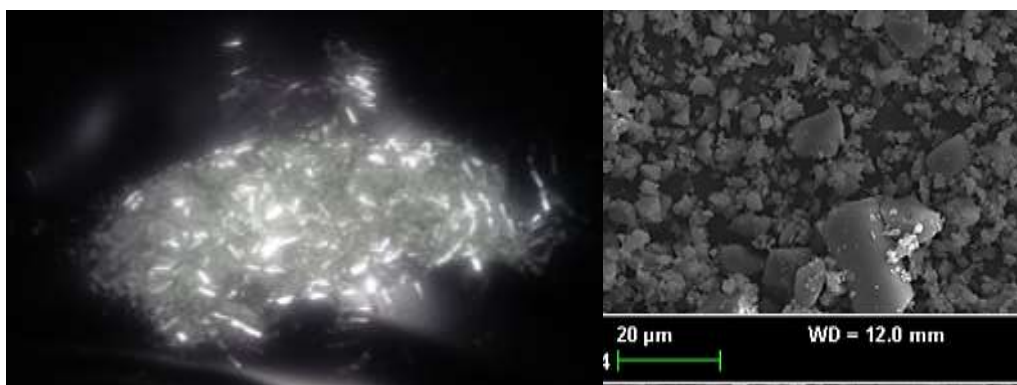
Fig-3: a) As received state of the glass fiber waste image, b)SEM-SE image of waste glass fiber,1000x
