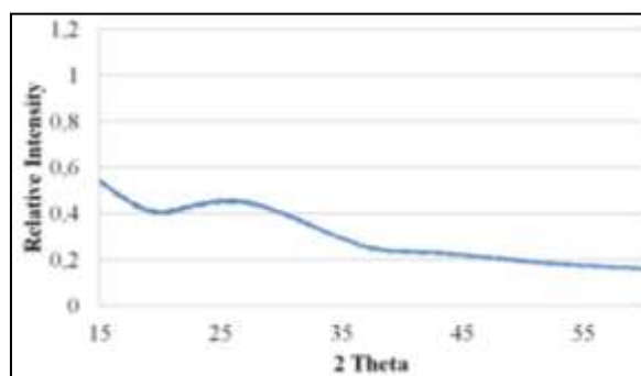
Fig-4: X-ray diffraction pattern of waste glass fiber
